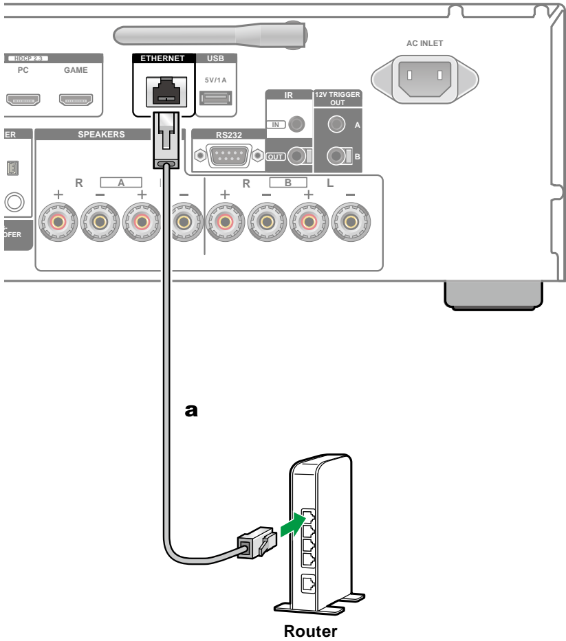
a Ethernet cable
