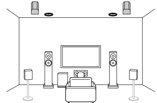
5.1.4 ch (Top Front and Rear High) ( →p34)
