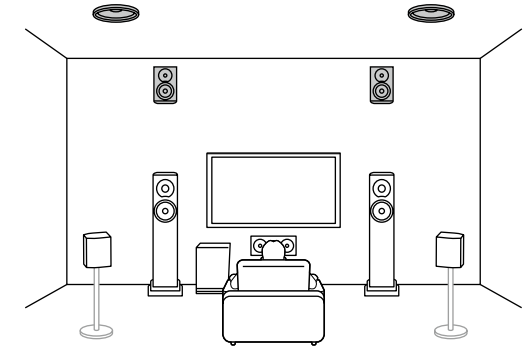
5.1.4 ch (Front High and Top Rear) ( →p34)
