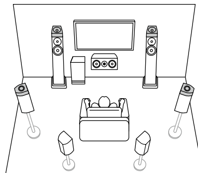
7.1.4 ch (Dolby Enabled Speakers (Front and Surround)) ( →p35)
