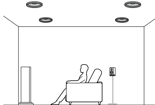
5.1.4 ch (Top Front and Top Rear) ( →p30)
