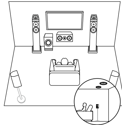
5.1.4 ch (Dolby Enabled Speakers (Front) and Top Rear) ( →p30)
