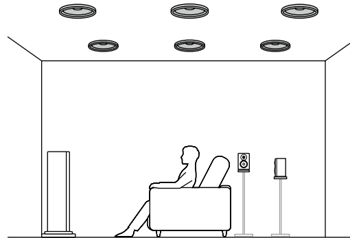
7.1.2 ch (Top Front or Top Middle or Top Rear) ( → p29 )
