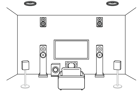
5.1.4 ch (Front High and Top Rear) ( →p30)
